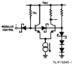
TL/F/5240-7
