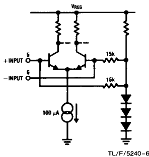
TL/F/5240-6
